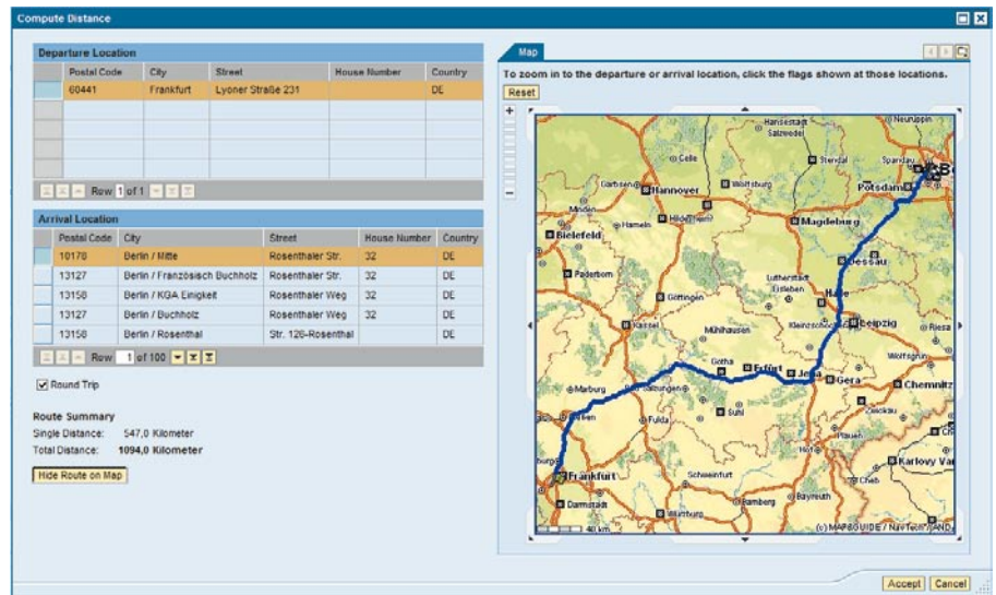
Routing with exact distance calculation
